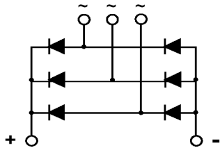
Circuit configuration:Three Phases Bridge
